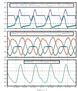
13. Comparison of simulation and measurement results for standard control system and fault-tolerant control system with extended AW, modifi u (flat-top modulation), and optimally injected d -current. (a) Experiment ( E_1 ): Comparison of simulation and measurement results for standard control em: \text{THD}_{i_d} = 41.8\% (simulation) versus \text{THD}_{i_d, \text{meas}} = 45.4\% (measurement). (b) Experiment ( E_2 ): Comparison of simulation and measurement results for fault-tolerant control system with extended AW, modifi u (flat-top modulation), and optimally injected d -current.
