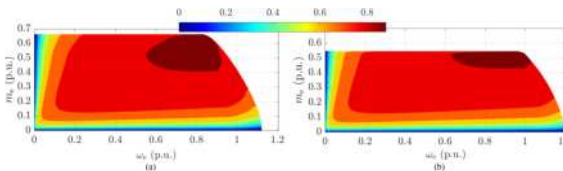
postfault efficiency maps of (a) 1N and (b) 2N connections within the (m_e, \omega_e) range of the proposed optimization in Section III-C
